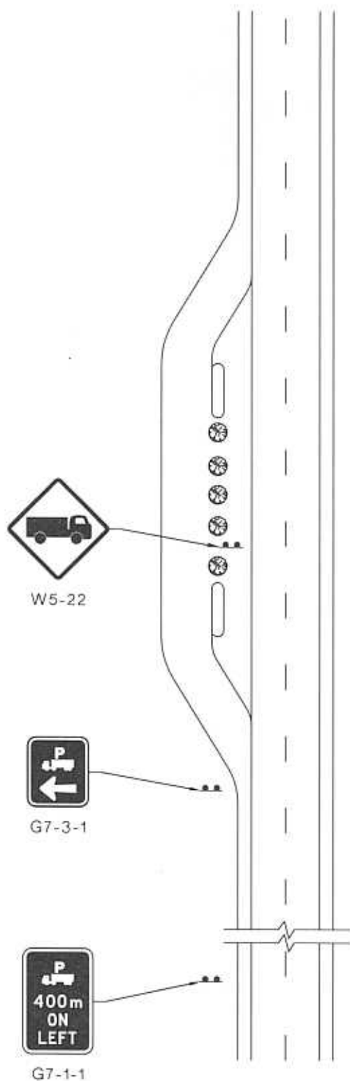
FIGURE 5.3 TRUCK PARKING AREA
